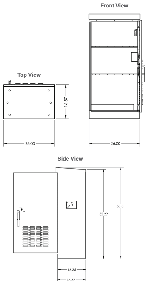
53" ZincBlue2 Cabinet
