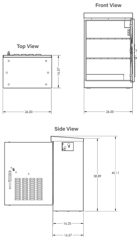
40" ZincBlue2 Cabinet
